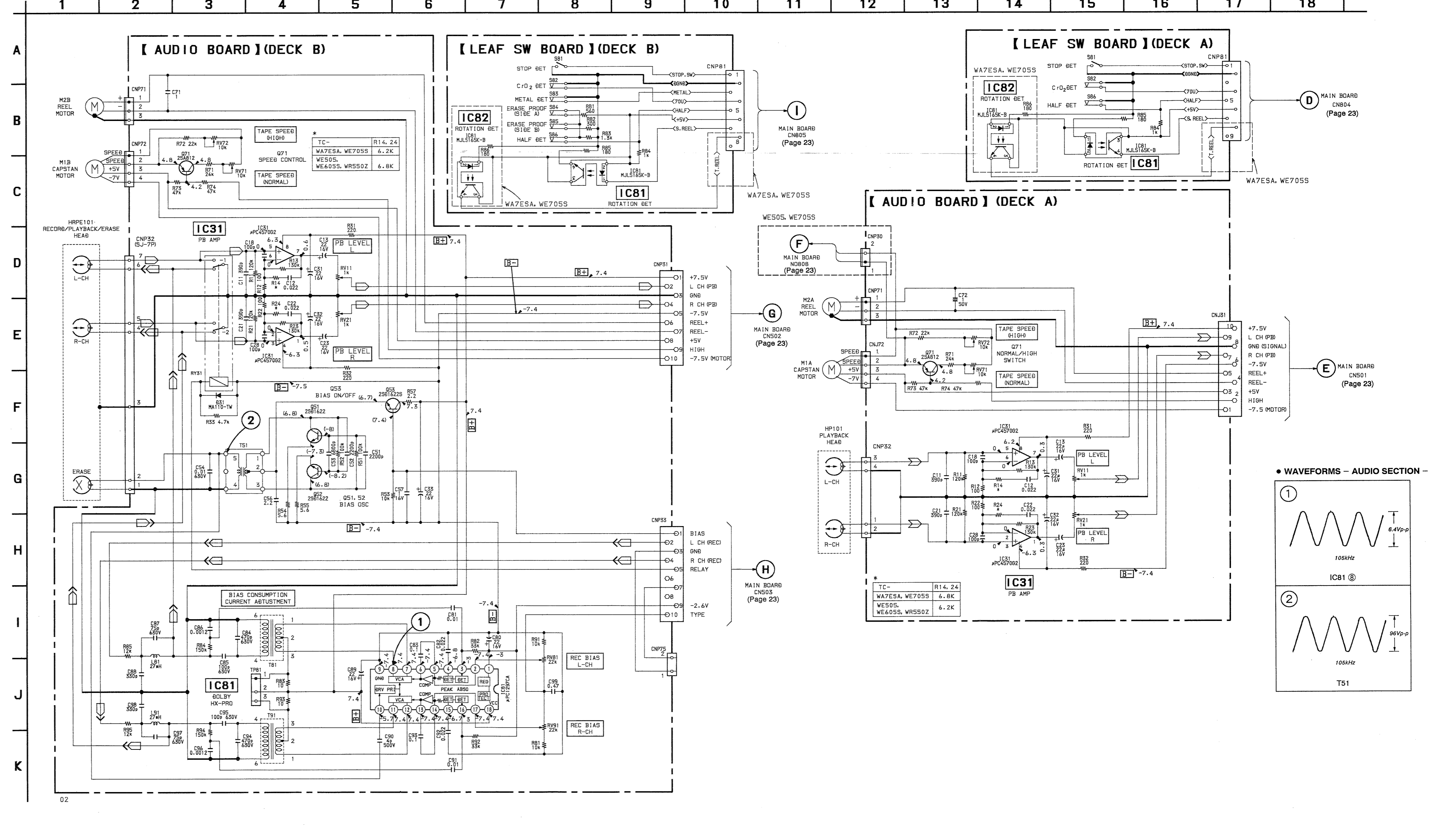
5-5. SCHEMATIC DIAGRAM (AUDIO SECTION)
