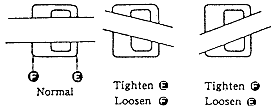
(The erasehead as seen when erasing the mirror cassette.)
