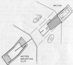
Detail 2C
