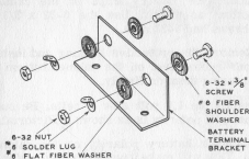
Detail 3A
